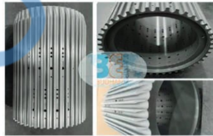
Infeed Drum
